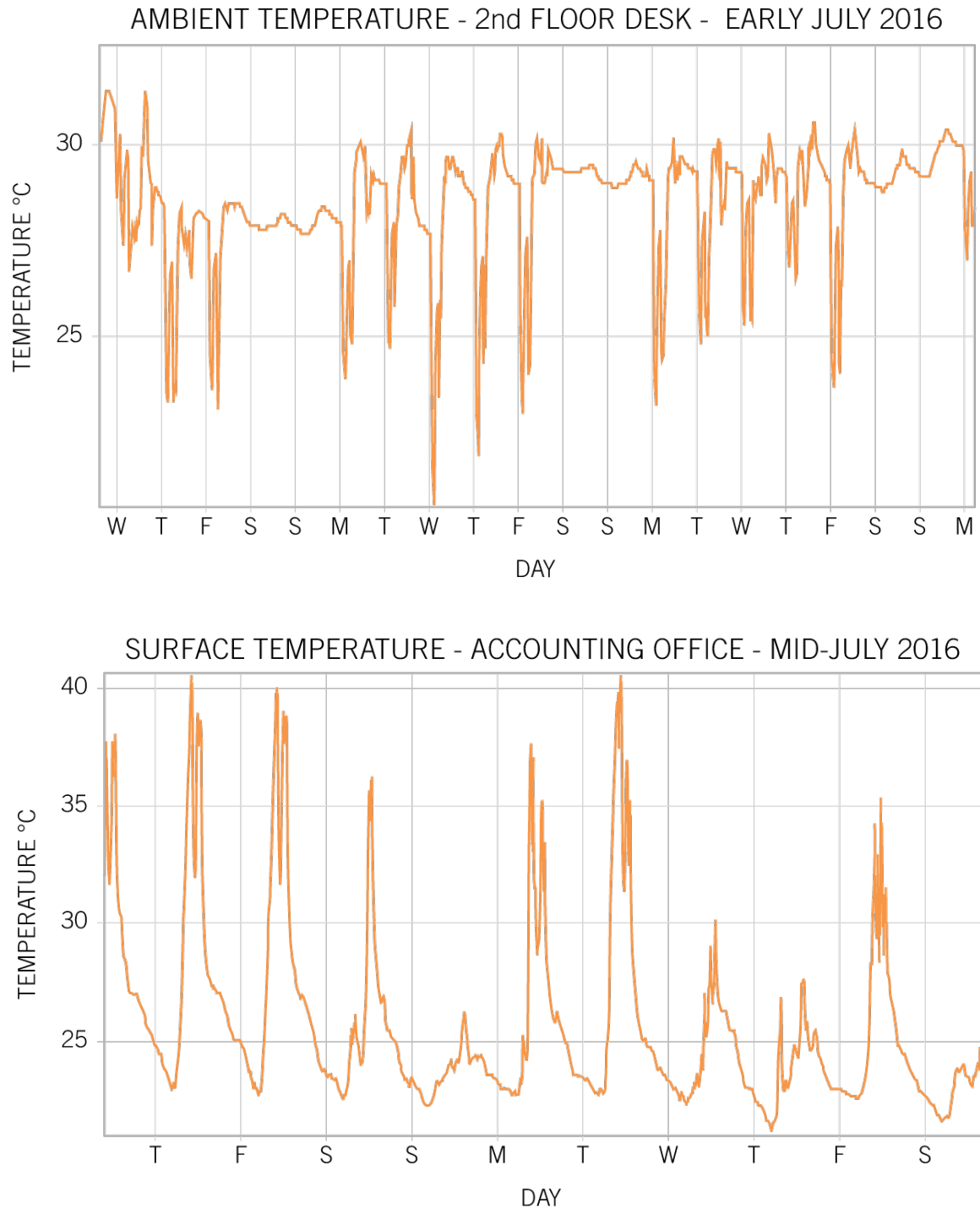
Figure 8: Collected temperature data over time from a desk and accounting office in the Vancouver studio of Perkins and Will. The troughs during the week are the building exhaust flushes, which influence only ambient temperature and not areas exposed to direct sunlight.
