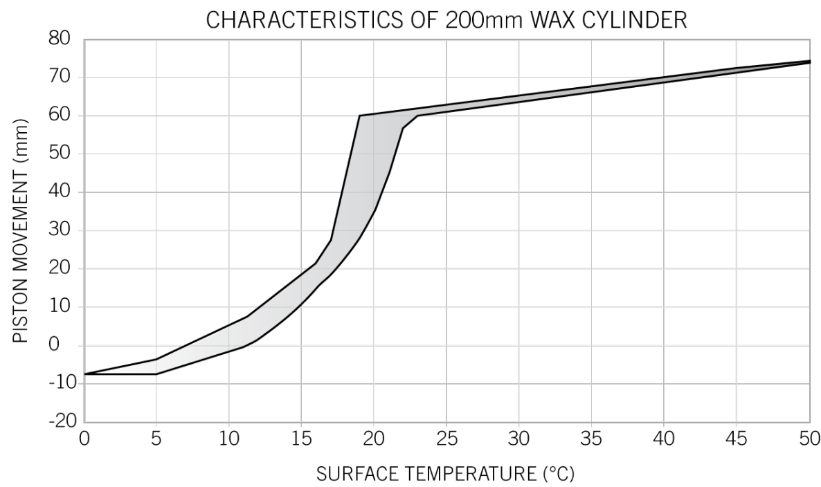
Figure 10: A sample response profile for a thermal actuator given in a temperature range. The response can vary, and is represented by an area (Adapted from E20D profile)°.
