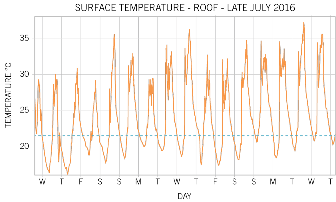
Figure 9: Surface temperature data from the roof of the Vancouver studio of Perkins and Will. The area above the line demonstrates where the actuator profiled below would be mostly closed.
